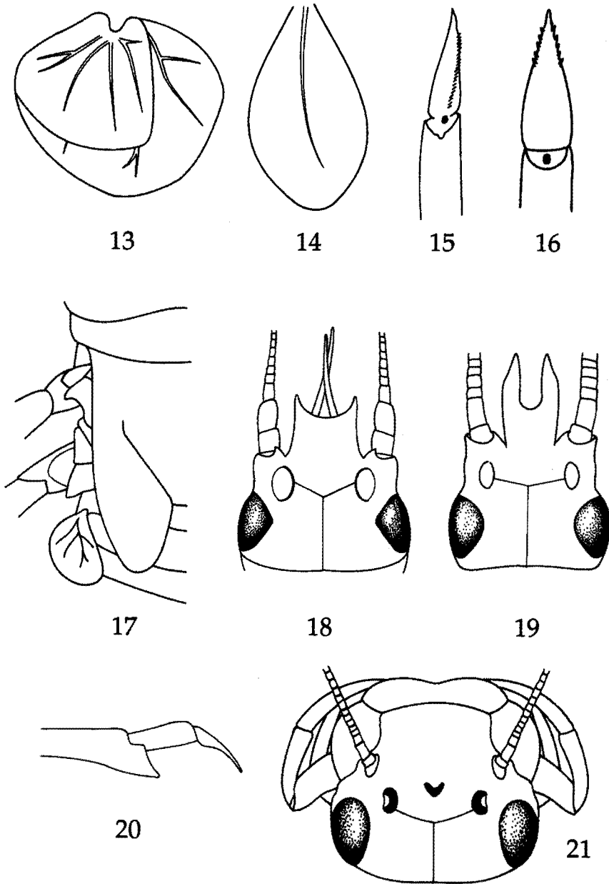
Figures 13–21 13, double abdominal gills of Cloeon sp.; 14, single abdominal gill of Baetis sp.; 15, ventral aspect of pretarsus of Baetis sp.; 16, ventral aspect of pretarsus of Centropetella sp.; 17, left side of thorax of Compsoeuriella sp. showing supracoxal projections above meso- and metathoracic legs.; 18, dorsal aspect of head of Ephemera ( Ephemera ) sp.; 19, dorsal aspect of head of Ephemera ( Dicrephmera ) sp.; 20, distal end of mesothoracic leg of Ephemera ( Ephemera ) sp.; 21, dorsal aspect of head of Choroterpides sp.
