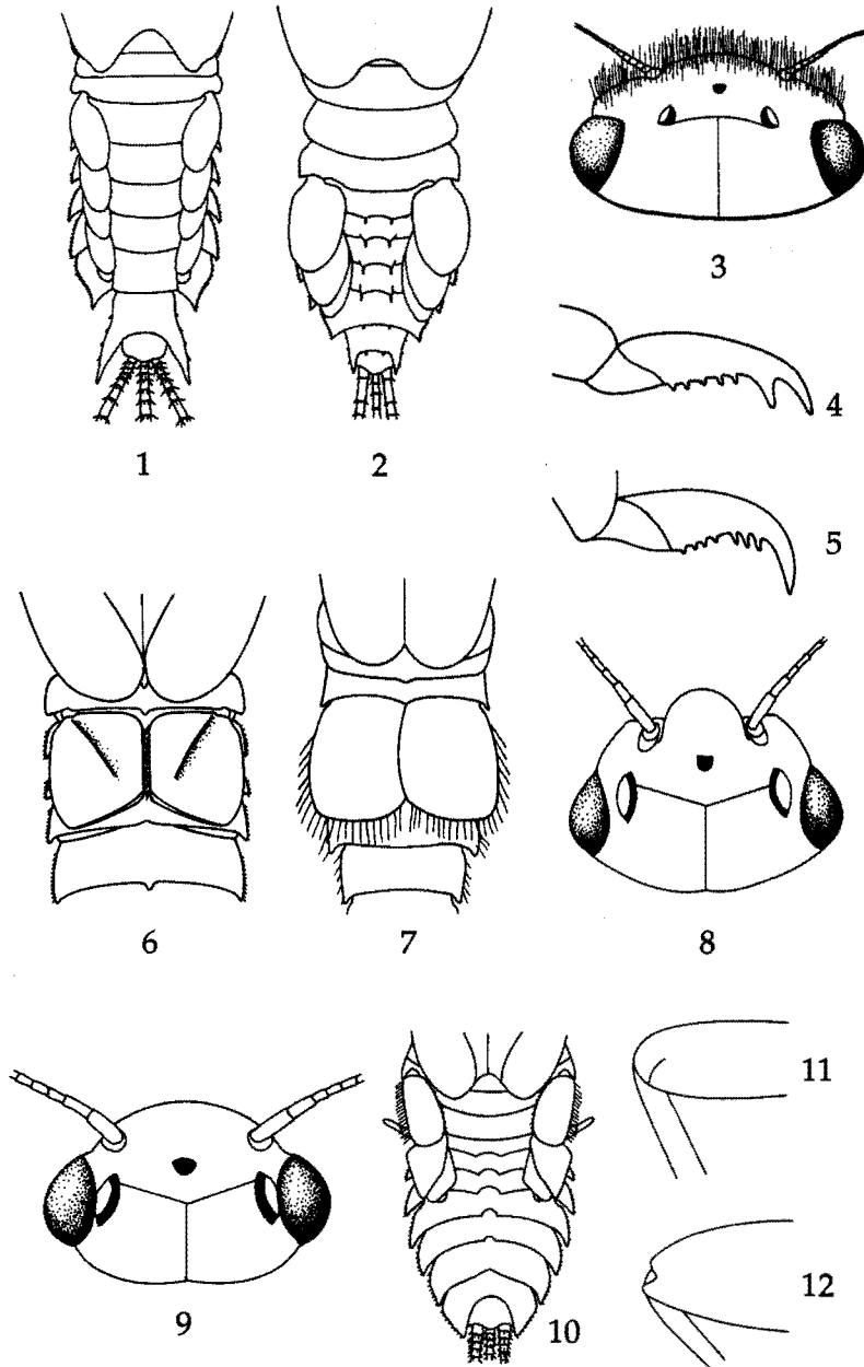
Figures 1–12. 1, dorsal aspect of abdomen of Crinitella permkami ; 2, dorsal aspect of abdomen of Serratella sp.; 3, dorsal aspect of head of Crinitella permkami ; 4, lateral aspect of tarsal claw of Teloganopsis sp.; 5, lateral aspect of tarsal claw of Serratella sp.; 6, operculate gills of Potamanthellus sp.; 7, operculate gills of Caenis sp.; 8, dorsal aspect of head of Clypeocaenis sp.; 9, dorsal aspect of head of Caenis sp.; 10, dorsal aspect of abdomen of Teloganella sp.; 11, distal end of femur of Baetis sp.; 12, distal end of femur of Afronurus sp.
