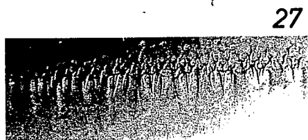
FIGS. 10-21 through 10-27. Thalerosphyrus josettae n. sp. 21: labrum; 22: hypopharynx; 23: labium; 24: maxilla; 25: median pectens of galea-lacinia; 26: spines on dorsum of hind femora; 27: posterior margin of tergite V.
