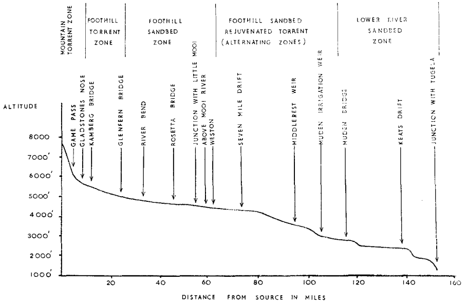
FIGURE 4. PROFILE DIAGRAM OF THE MOOI RIVER
