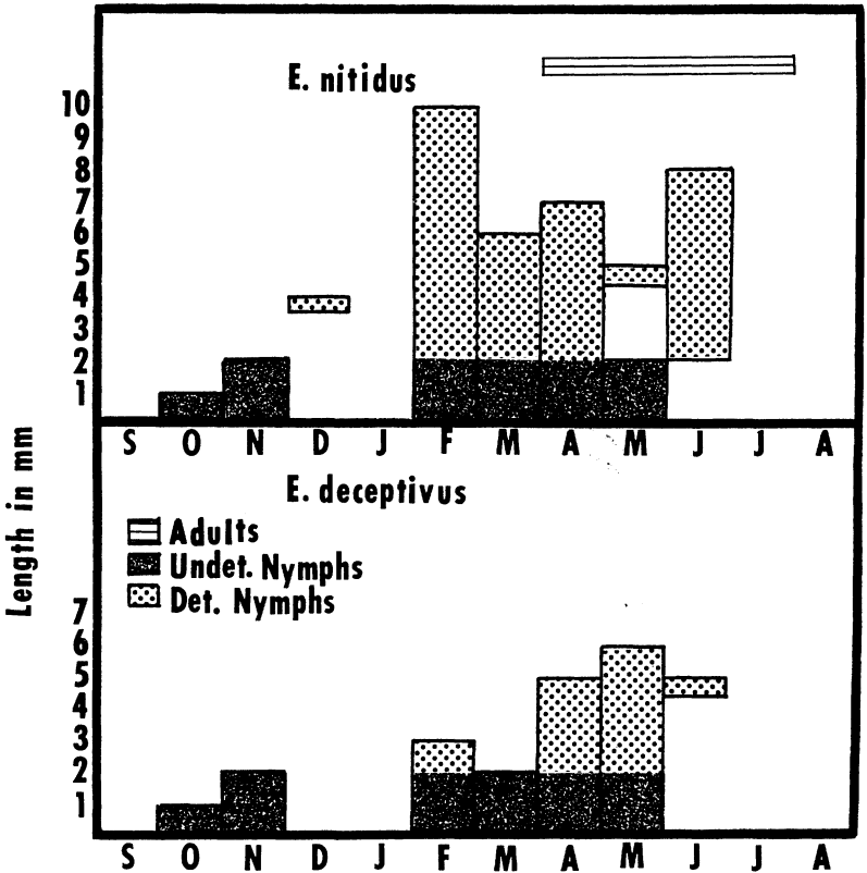
FIG. 2. Seasonal occurrence and size ranges of Epeorus ntidus and E. deceptiveus in Oak Creek, Benton Co., Oregon. The < 2 mm group was not identified to species and has been repeated for each.
