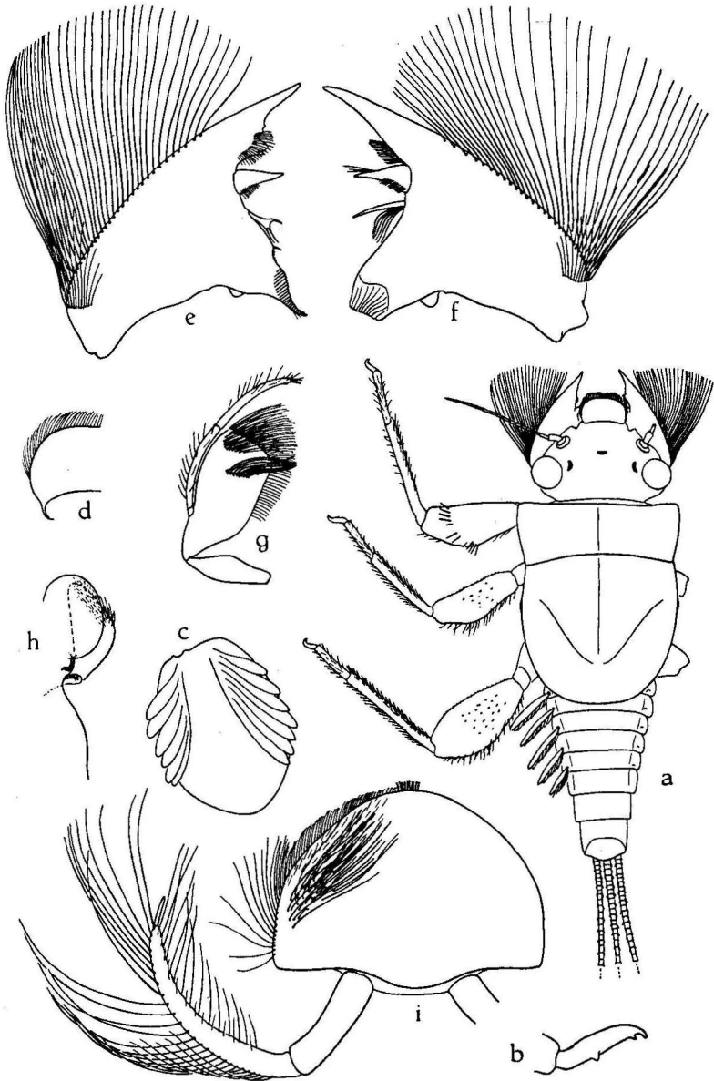
Fig. 1. — ? Tricorythus sp., larve.
